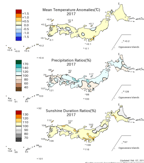
Figure 7 Annual climate anomalies/ratios for Japan in 2017
