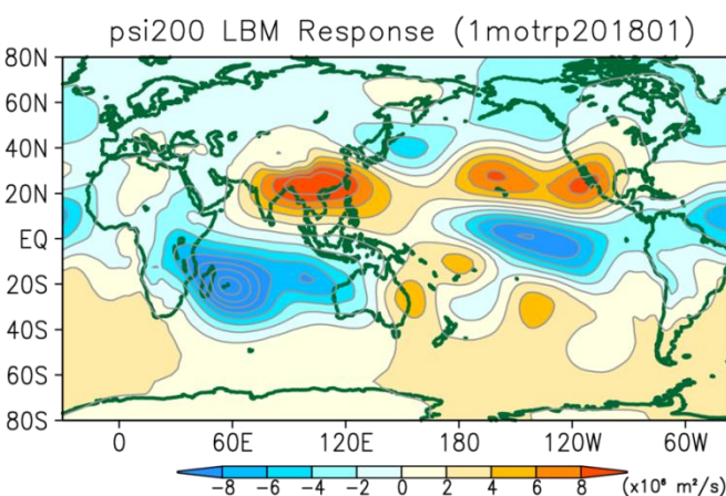
Figure 16 Atmospheric response (stream function at 200 hPa) in the LBM experiment using diabatic heating over the tropics for January 2018
