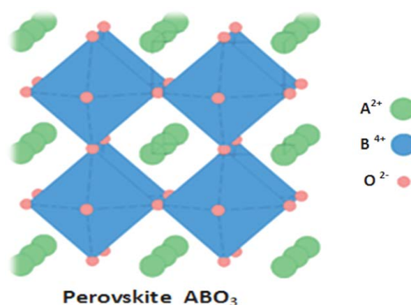
Fig. 2. Crystal structure of perovskite ABO 3 .
