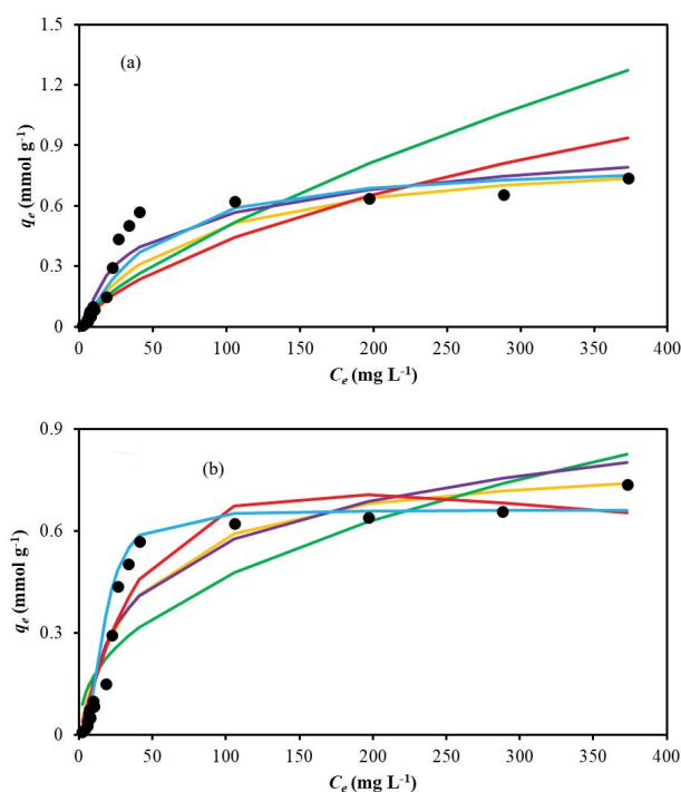
Fig. 6. Comparison of experiment isotherm data (●) with Langmuir (—), Freundlich (—), Temkin (—), Redlich–Peterson (—), and Sips (—) isotherm models.
