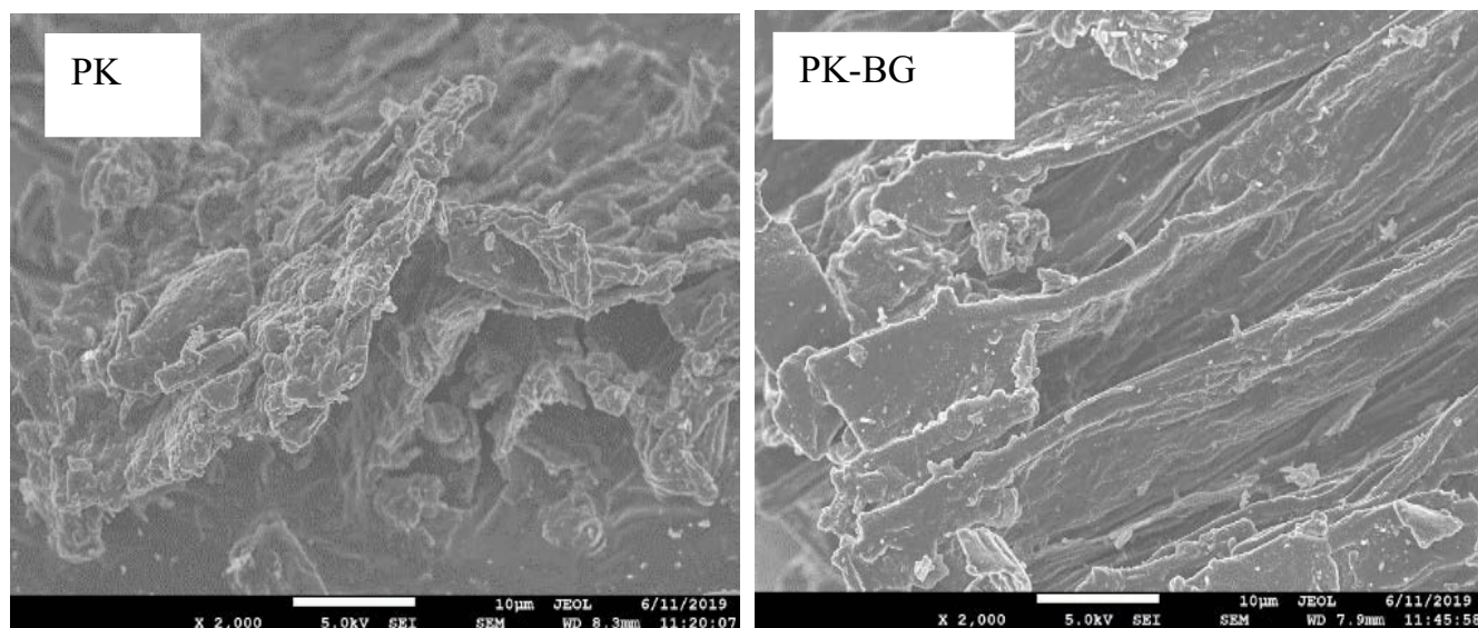
Fig. 2. SEM images of Pakis before and after adsorption of BG at 2,000× magnification.
