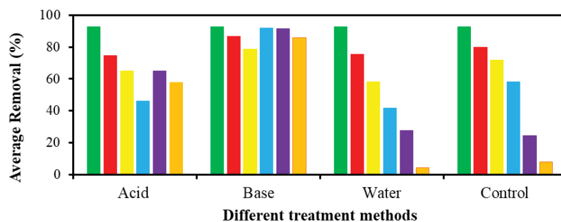
Fig. 9. Regeneration of spent MKL for the adsorption of BG in five consecutive cycles [cycles 0 (■), 1 (■), 2 (■), 3 (■), 4 (■), and 5 (■)].
