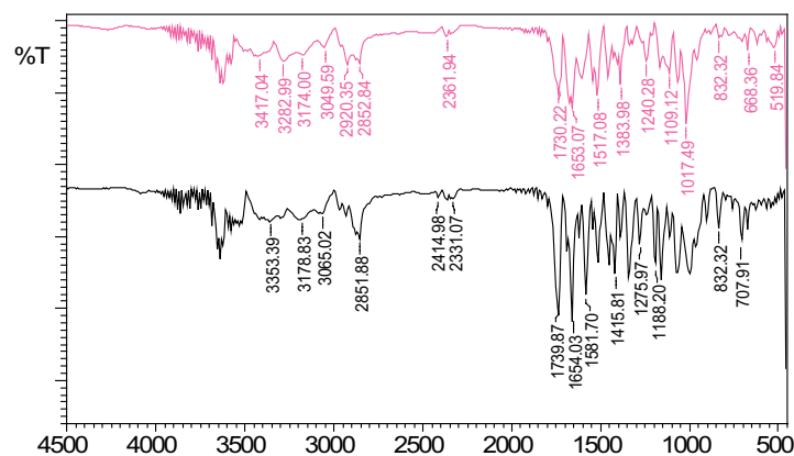
Fig. 1. FTIR spectra of Pakis before (black) and after (pink) adsorption of BG.
