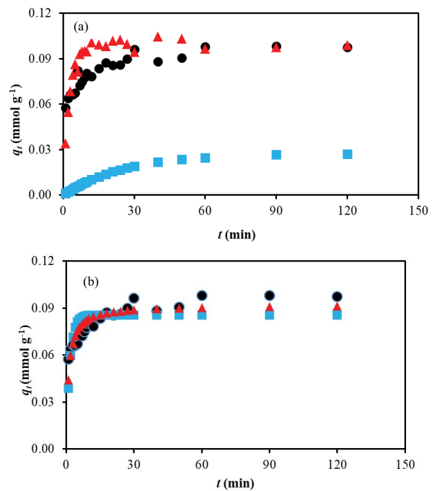
Fig. 5. Comparison of experiment kinetics data (●) with Lagergren pseudo-first-order (■) and pseudo-second-order (▲) models using (a) linear regression and (b) nonlinear regression analyses.
