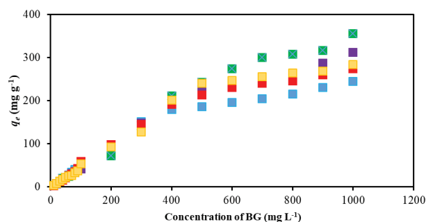
Fig. 8. Adsorption of BG onto Pakis at 298 K (■), 313 K (■), 323 K (■), 333 K (■), and 343 K (■).
