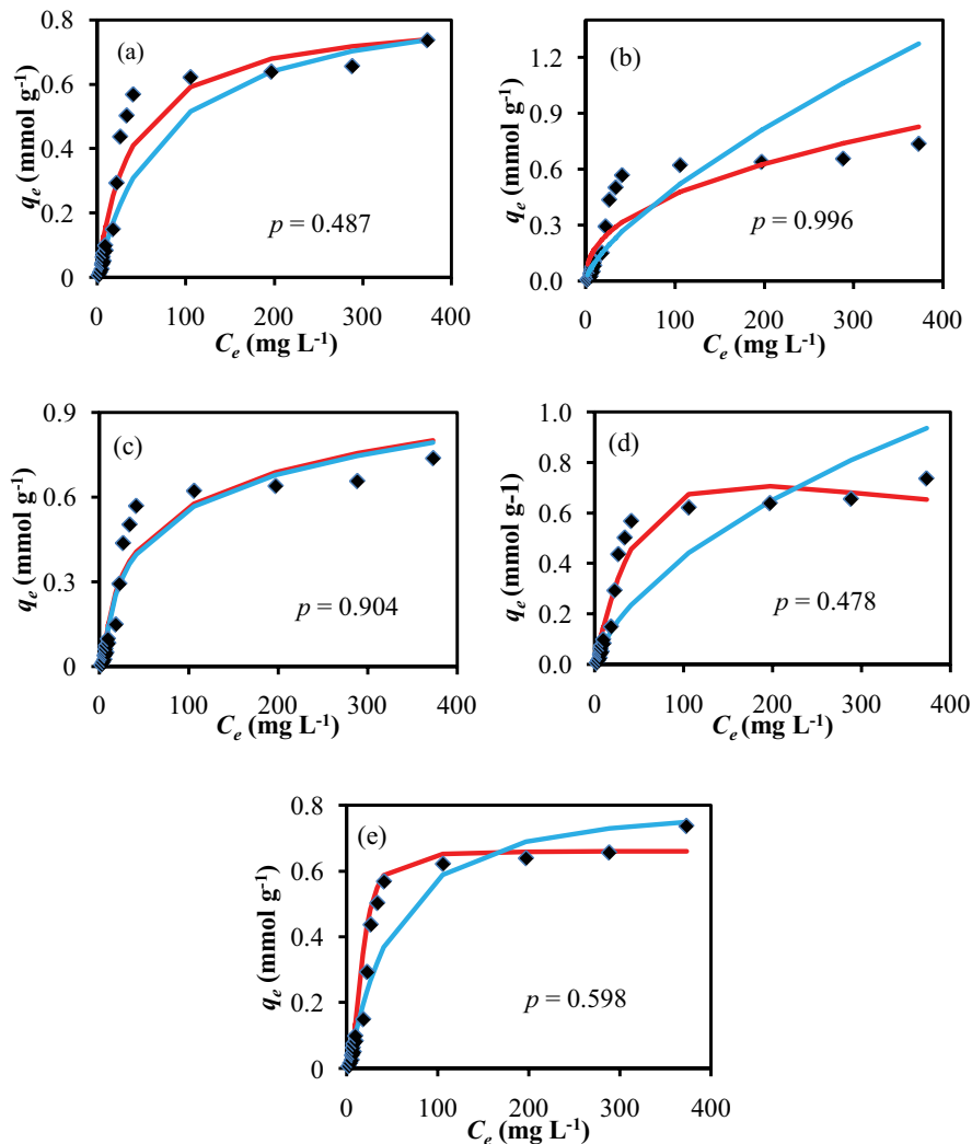
Fig. 7. Comparison of experiment data (◆) for (a) Langmuir, (b) Freundlich, (c) Temkin, (d) Redlich–Peterson, and (e) Sips isotherm models with linear (—) and nonlinear (—) regression analyses with the p values using ANOVA for adsorption of BG onto Pakis.
