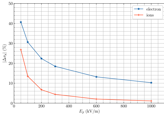
Fig. 4. Error on the profile measurement, for electrons and H_2^+ ions, due to space charge effects versus the extraction field. The beam is assumed to be a Gaussian with \sigma_x = \sigma_x = \sigma_x = 2 mm
