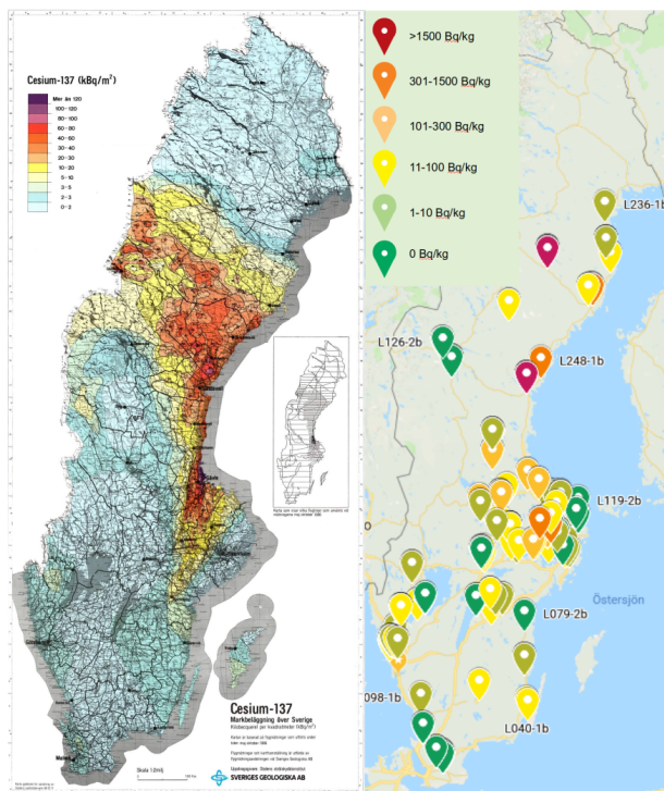
Figure 4. The results of the airborne measurements of ^{137}\text{Cs} in \text{kBq}/\text{m}^2 , performed by the Geological Survey in Sweden in 1986 (left) [11], and a Google Maps visualization of the distribution of collected fungi samples in the citizen science project, color-coded for activity in \text{Bq}/\text{kg} (right) [10]. For better view, follow the links given in the references.
