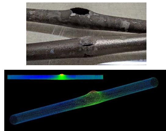
Fig. 8. Post-test examination results. Top: final aspect of burst dummy rods (pre-oxidised Zircaloy cladding, Al 2 O 3 pellets, after several ramps). Bottom: 3D post-test laser metrology.
