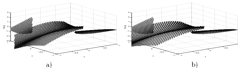
Figure 2: a) The function (5); b) its estimate after the network initialization.
