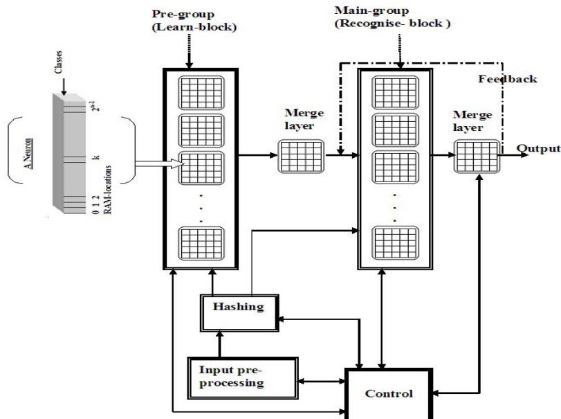
Figure 1: A simplified schematic of Hardware Architecture of EPCN network.
