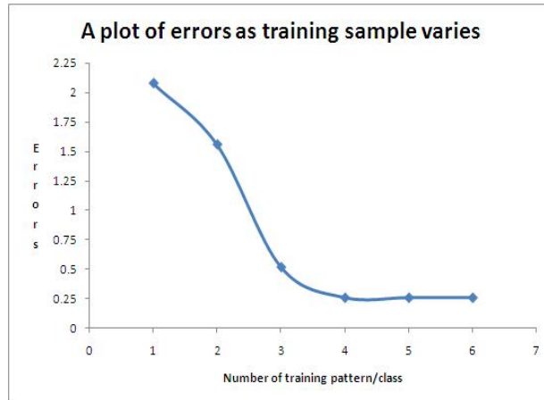
Figure 4: Summary of results obtained by varying the number of pattern per class used during learning.
