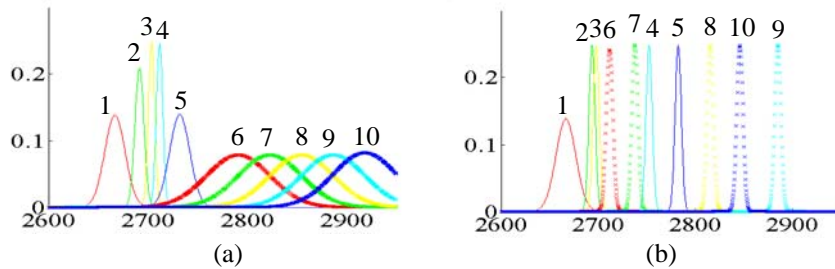
Fig 2. Example of neuron gathering in Gaussian layer. Neurons associated with the reactor pressure measurements, the pressure scale is [2600 kPa, 2950 kPa]. (a) after 3h learning. (b) after 80h learning. The number attached to each curve corresponds to the number of the corresponding neuron on the hidden layer.
