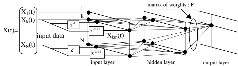
Fig 1. Neural network structure for data mapping
