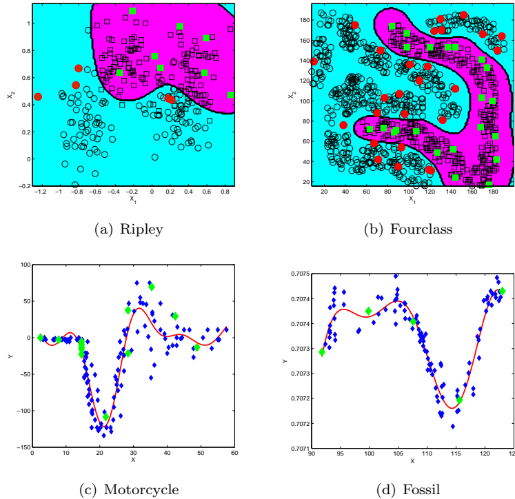
Fig. 1: Examples of sparse models (decision surfaces in classification and red lines in regression) obtained by ISLS-SVM.
