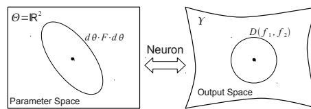
Figure 2: Established differentiable relation (Neuron) and metrics F and D between parameter space \Theta = \mathbb{R}^2 and manifold of possible output distributions \Upsilon .
