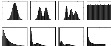
Figure 1: Four different input distributions f_x(x) (1. row) and the corresponding learned exponential-like output distributions f_y(y) for \mu = 0.2 (2. row).
