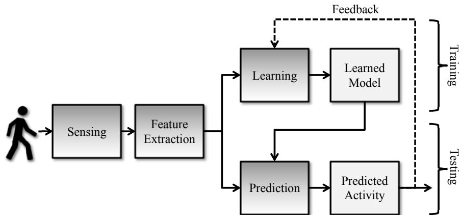
Fig. 1: The Human Activity Recognition Process Pipeline.
