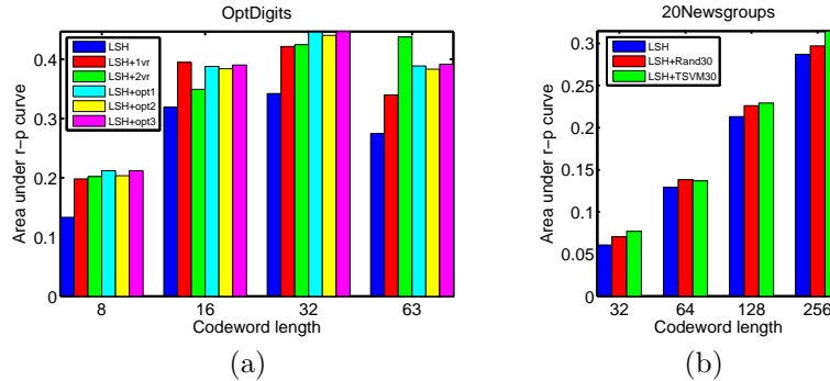
Fig. 1: Area under the precision–recall curve for various code lengths: (a) Opt-Digits, (b) 20Newsgroups data set.
