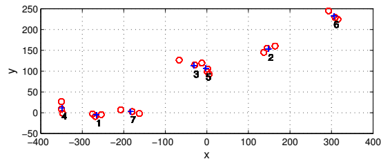
Fig. 2: Reproduction of the learned sequence of starting points (in mm). Circles mark the starting points of the training data and the cross mark the reproduced starting point of the MP indexed by 1 – 7.
