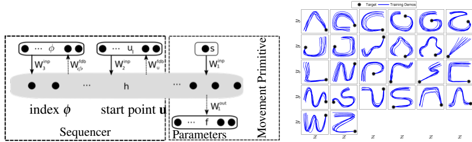
Fig. 1: Left: A flat representation of a sequence of starting points \mathbf{u}_l and indices \phi together with the MP itself. Right: LASA data set of handwriting motions for training.
