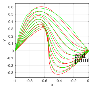
Fig. 4: Two motions interpolated through mixture coefficients at indexing input (red/dark) vs. MP with external computed sum of forces (green/light).
