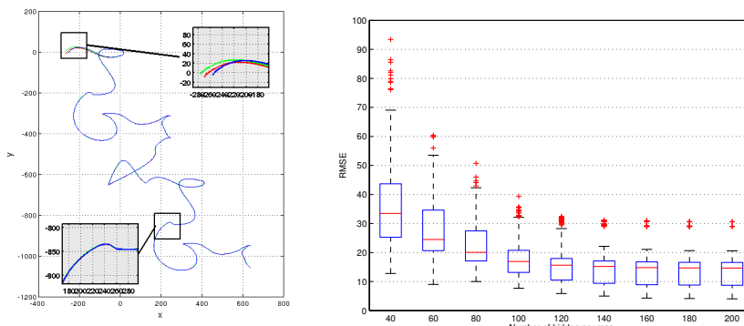
Fig. 3: Left: Sequencing seven MPs (Fig. 4) repeated twice. Three runs started from different initial points ( zoomed). Right: Error for learning of M = 20 motion patterns with different hidden layer sizes.
