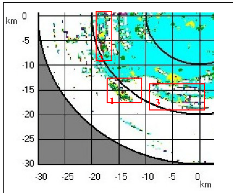
Fig. 9: Detailed Doppler measurements observed for 3 wind farms located south-east from French radar of Abbeville.
