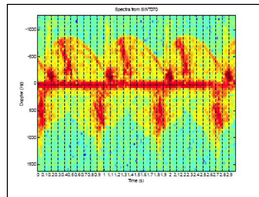
Fig. 1.b: Time variation (3s) of the Doppler spectrum of an Enercon E66 wind mill for a 39° rotor orientation (QuinetiQ, 2003).
