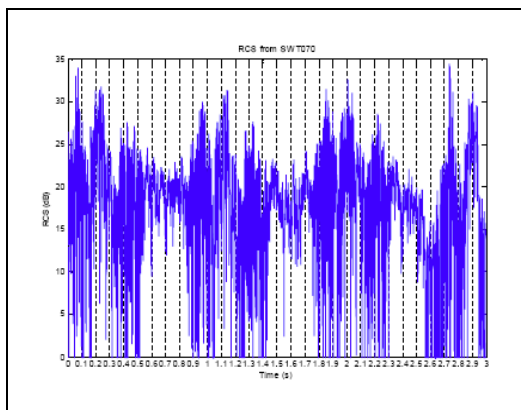
Fig. 1.a: Time variation (3s) of 3 GHz RCS of an Enercon E66 wind mill for a 39° rotor orientation (QuinetiQ, 2003).
