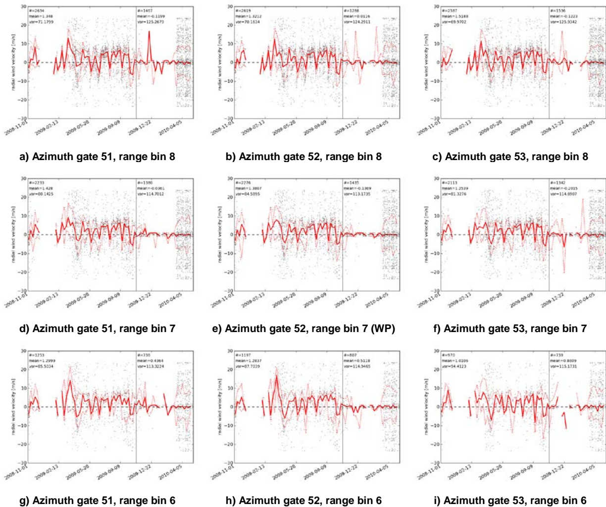
Fig. 10: As Figure 5 but for radial wind velocities.
