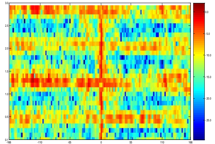
Fig. 12: Falaise 8 October 2008 13h35. Time evolution (3s) of the Doppler spectrum from a wind mill located 19 km from French radar of Falaise. The color scale represents the values of amplitude of the received power in dB relative to the maximum observed over the measurement period. The central axis (0Hz) corresponds to echoes associated with non-mobile elements present in the measurement volume.
