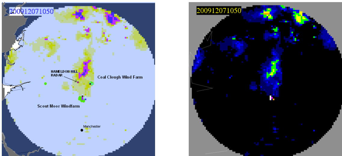
Fig. 7: Wind turbine clutter in the precipitation (left) and reflectivity imagery (right) for the Hameldon Hill radar (UK) on 7 December 2009 1050 UTC. The resolution is 1 km. Images kindly provided by S. Holton (UKMO).
