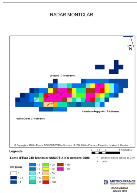
Fig. 4: Wind farms in Salles-Curan, Castelnau-Pegayrols and Lévezou located between 19 and 31 km from the French radar of Montclar produce an impact zone on precipitation accumulation data extending 25 km long and 5 km width. It renders data unavailable over an area of about 125 km 2 .
