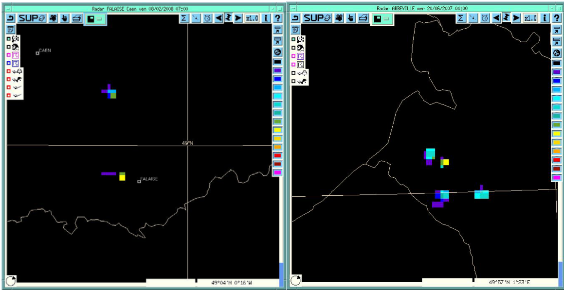
Fig. 2: Observation on 8 February 2008. Disturbance of precipitation data in vicinity of the French radar of Falaise. North, wind farm of Conteville at a distance of 19,9 km from the radar. South, wind farm of Aubigny Soulangy at a distance of 3.5 km from the radar.
