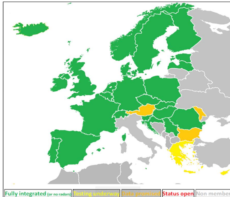
Fig. 1: Countries sending reflectivity data to OPERA Data Center (situation in June 2018).
