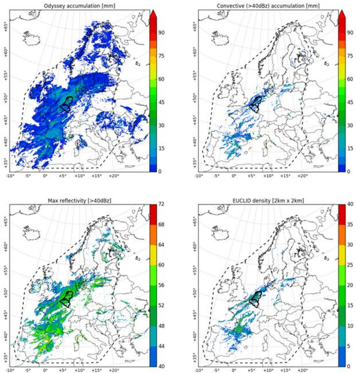
Fig. 5: Different panels depict three types of daily maps as derived from the ODC reflectivity/rainrate data as well as the EUCLID lightning density over Europe on 2015/08/31. EUCLID lightning observations are restricted within the dashed-dotted polygon.
