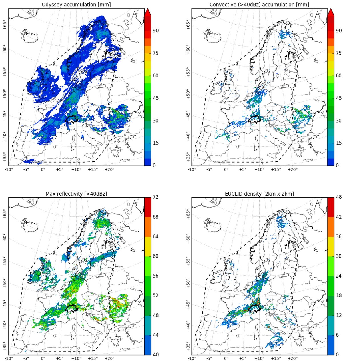
Fig. 6 Different panels depict three types of daily maps as derived from the ODC reflectivity/rainrate data as well as the EUCLID lightning density over Europe on 2016/06/24. EUCLID lightning observations are restricted within the dashed-dotted polygon.
