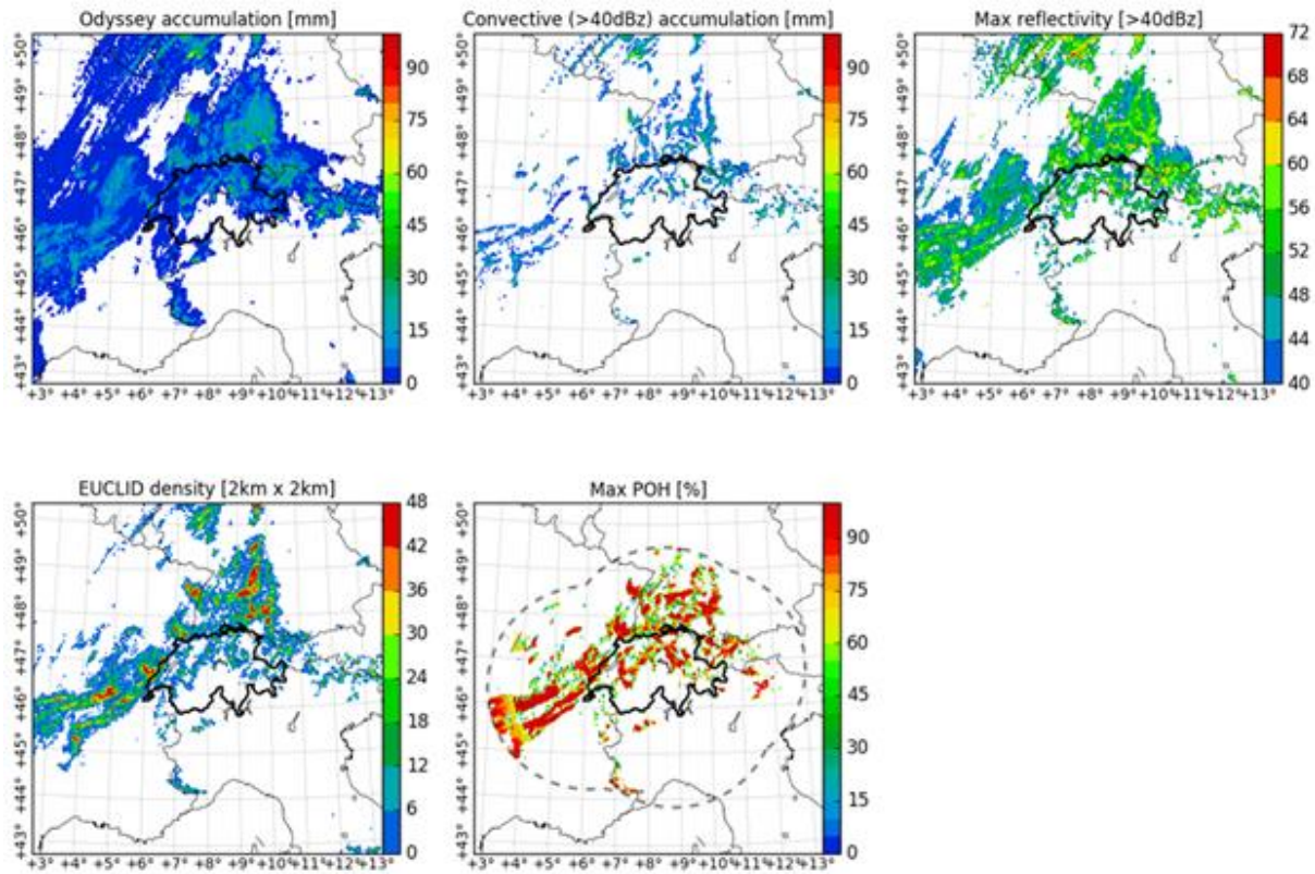
Fig. 4: Top panels depict different types of daily maps as derived from the ODC reflectivity/rainrate data centralized on Switzerland on 2016/06/24. Corresponding maps of the EUCLID lightning density and national POH of MeteoSwiss are plotted in the lower panels.
