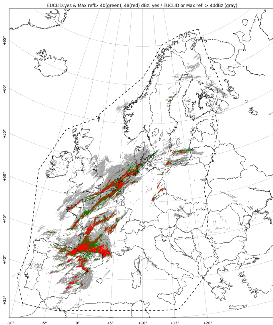
Fig. 7: Mapping of convective precipitation over Europe on 2015/08/31. Areas with lightning activity or max reflectivity larger than 40 dBZ are indicated in grey, whereas regions with lightning activity and max reflectivity larger than 40 and 48 dBZ are plotted in green and red, respectively. Note that EUCLID lightning observations are restricted within the dashed-dotted polygon.
