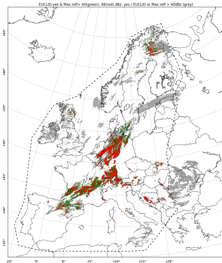
Fig. 8: Mapping of convective precipitation over Europe on 2016/06/24. Areas with lightning activity or max reflectivity larger than 40 dBZ are indicated in grey, whereas regions with lightning activity and max reflectivity larger than 40 and 48 dBZ are plotted in green and red, respectively. Note that EUCLID lightning observations are restricted within the dashed-dotted polygon.
