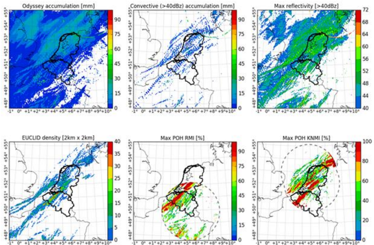
Fig. 3: Top panels depict different types of daily maps as derived from the ODC reflectivity/rainrate data centralized on the Benelux on 2015/08/31. Corresponding maps of the EUCLID lightning density and national POH of RMI and KNMI are plotted in the lower panels.
