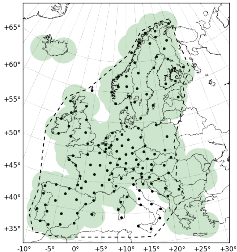
Fig. 2: Lightning detection sensor locations (dots) within the EUCLID network, as well as the EUCLID coverage (dashed line). The extent of the ODC coverage is indicated in green. As can be seen, there is a good match between the coverage of EUCLID and ODC.
