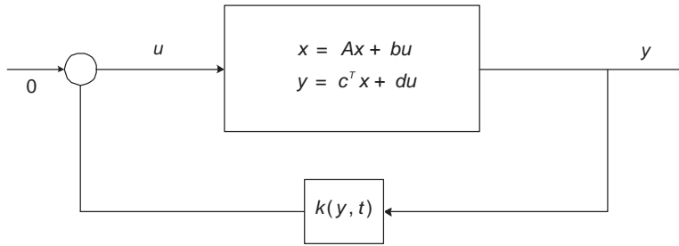
Figure 8: Graphical depiction of the Lur'e system. For the present discussion we consider SISO systems: A is a stable n \times n matrix, b , c are appropriately dimensioned vectors, and d is a scalar.
