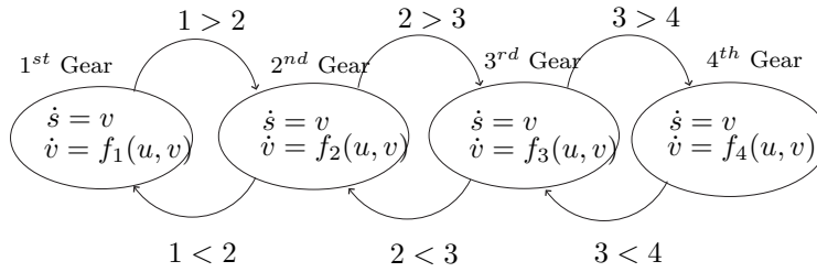
Figure 1: A hybrid model of a car with a manual gearbox [31, 74].
