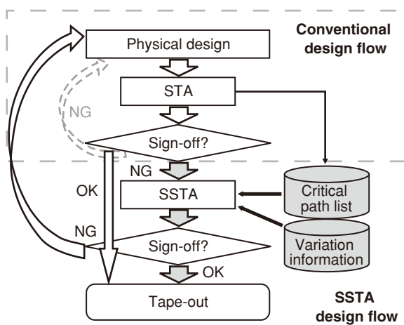
Figure 5 SSTA and conventional ASIC design flows.
