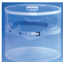
Figure 2. TLD-700H with headband on the surface of Cylindrical phantom
