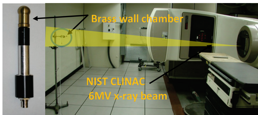
Figure 1. Setup of chamber in the megavoltage x-ray beam
