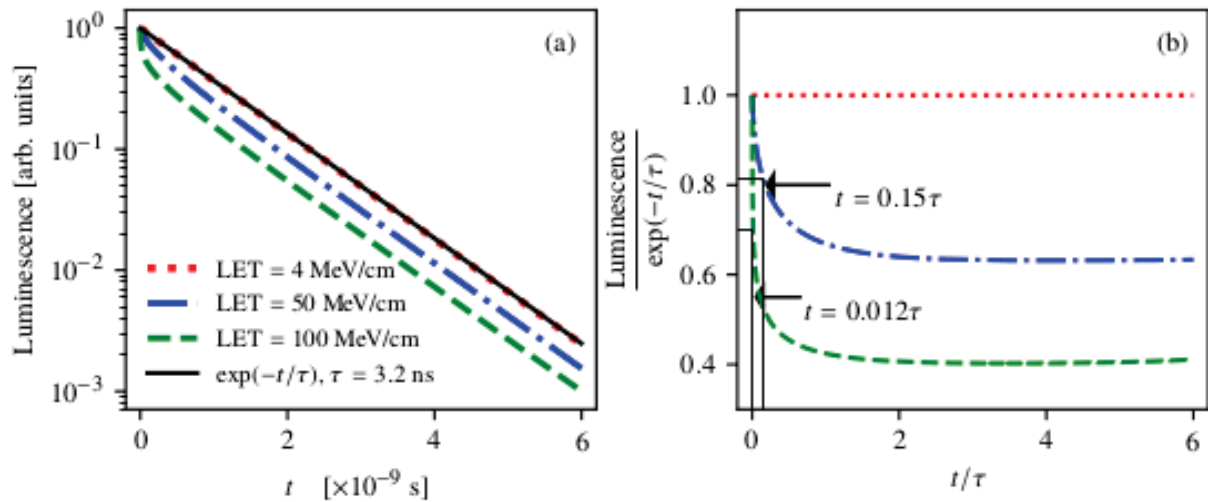
Figure 1. (a) The luminescence from 3 protons with different LET in a plastic scintillator. (b) The ratios of the luminescence to the quenching-free exponentially decaying scintillator signal.
