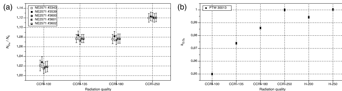
Figure 1. a: experimental results of p_Q factors (convolved with (\square\square\square) water to air ratios that were averaged over the x-rays photon spectra) for five ionization chamber model NE2571 in four radiation qualities (data provided by CEA-LIST LNE-LNHB, stated uncertainties indicate a coverage factor of 1). b: Monte Carlo calculations of k_{Q,Q0} factors for the ionization chamber PTW 30013 in six radiation qualities (data provided by ENEA-INMRI and based on the code EGSnrc, uncertainties are type A only). Radiation qualities shown include four from the CCRI series [4] (a, b) and two qualities from the ISO 4037-1 norm (b).
