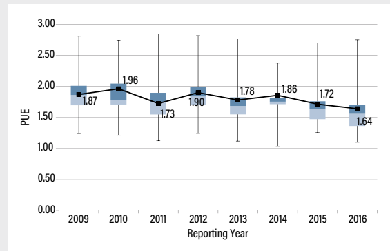
Figure 5. EU Code of Conduct participant reported PUE by year from Avgerinou et al (2017).
