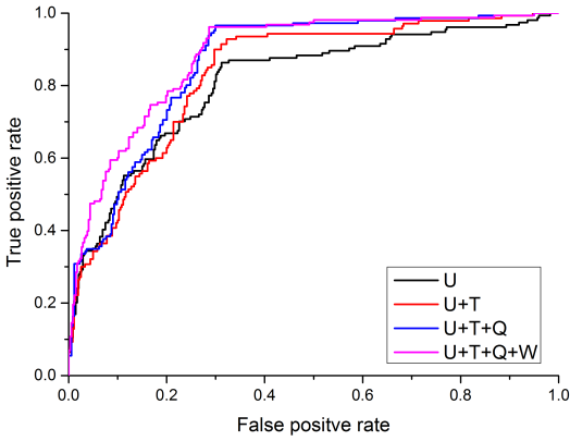
Figure 4: Comparison of ROC curves for detection methods from different sets of seed promotion channels
