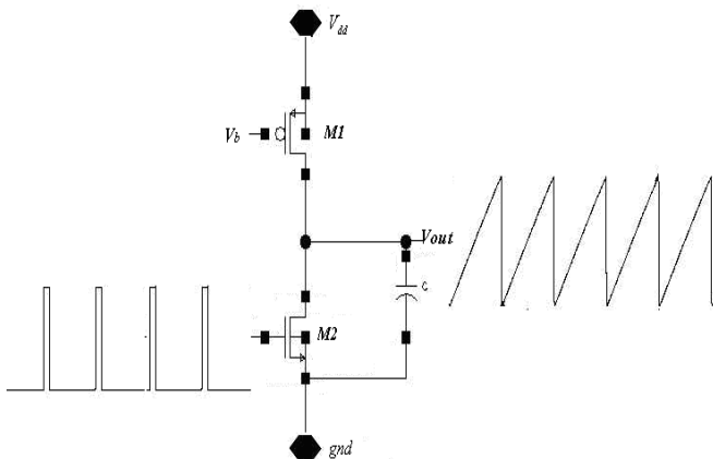
Fig3. Ramp Generation
