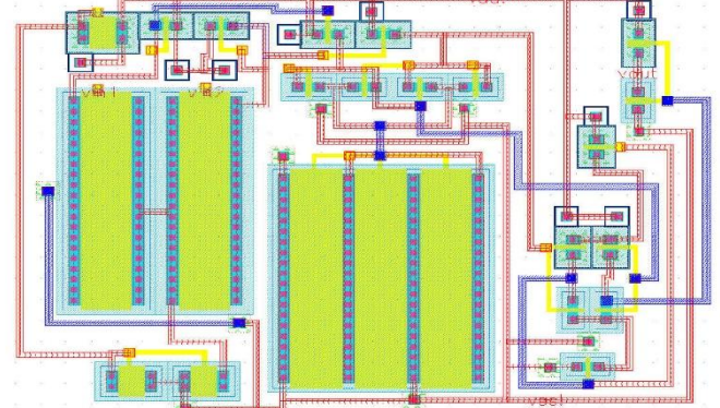
Fig.22. Layout of PWM comparator (27 μm × 19 μm)
