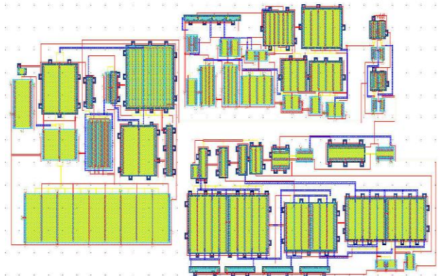
Fig.21. Layout of Ramp Generator ( 148 μm × 60 μm)
