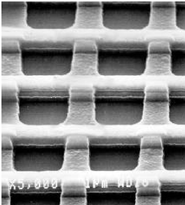
Figure 1. Scanning electron micrograph (SEM) of CCD polysilicon layers.
