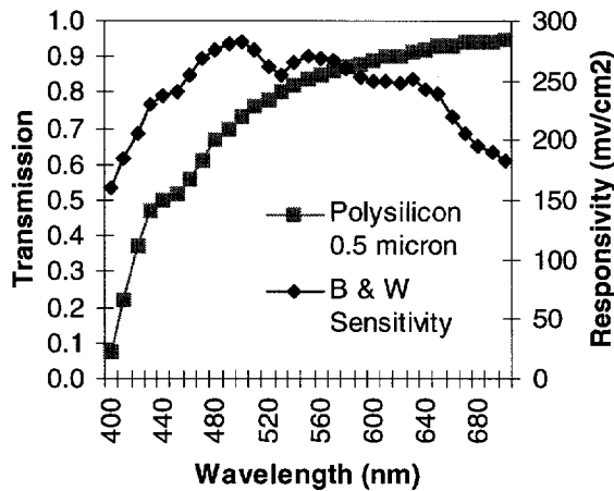
Figure 2. Spectral Transmission of 0.5 micron Polysilicon and B & W Sensitivity of CCD without microlenses.
