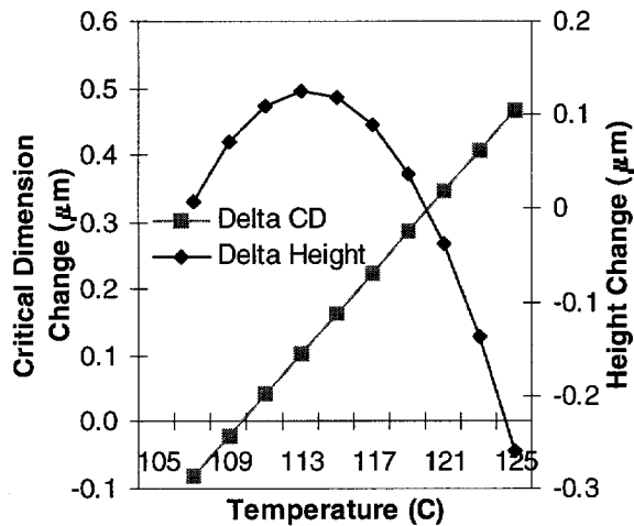
Figure 6 Changes in critical dimension and height for microlenses after a 2 minute hot plate reflow.
