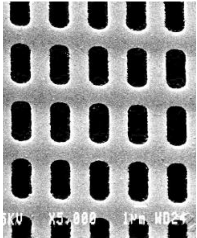
Figure 4. A top-view SEM of a 1500 angstrom thick pattern of apertures (shown in black) in chrome on quartz wafers. The color filters, focusing layers, conforming layers and microlenses are applied and patterned on these apertures for evaluation.
