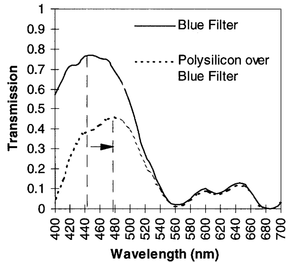
Figure 3. Blue light transmission through polysilicon.
