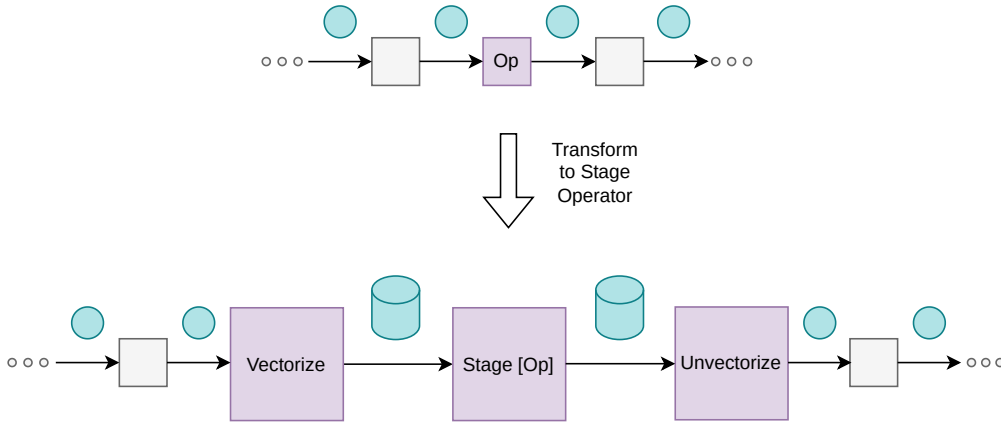
Figure 1: The Stage transformation changes the operator interface from tuple-at-a-time to buffer-at-a-time.
