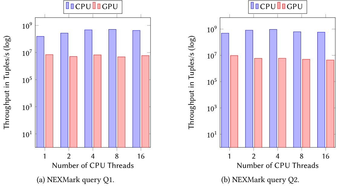
Figure 2: End-to-end query processing throughput for NEXMark queries Q1 (left) and Q2 (right). The stage buffer size is set to 64 MB.
