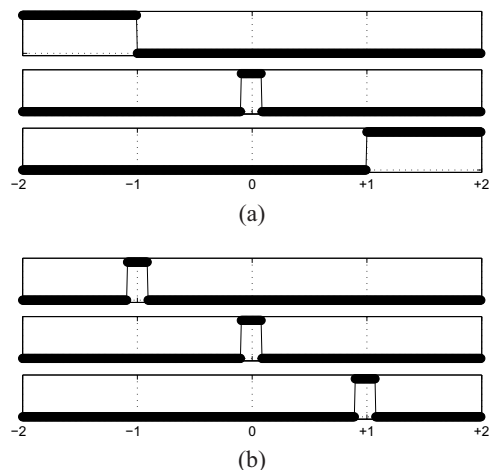
Figure 2: Left extremity filter, temporal support of the 5 central filters, and right extremity filter of the original (a) and of the modified (b) filterbank. The x -axis is in octaves per 8 ms.
