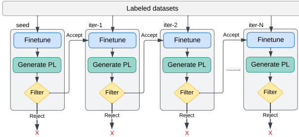
Figure 1: Overview of proposed self-training approach.
