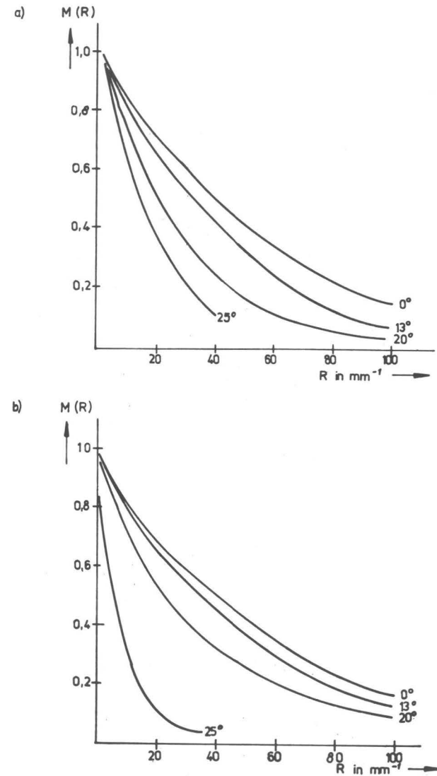
Fig. 6: Lametar 8/200 - MTF curves for white light at different angles and f/8
