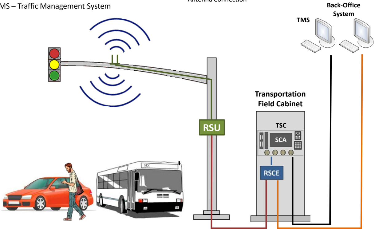
Figure 3. Example of an RSU mounted on a pole with antennas mounted on the mast arm
