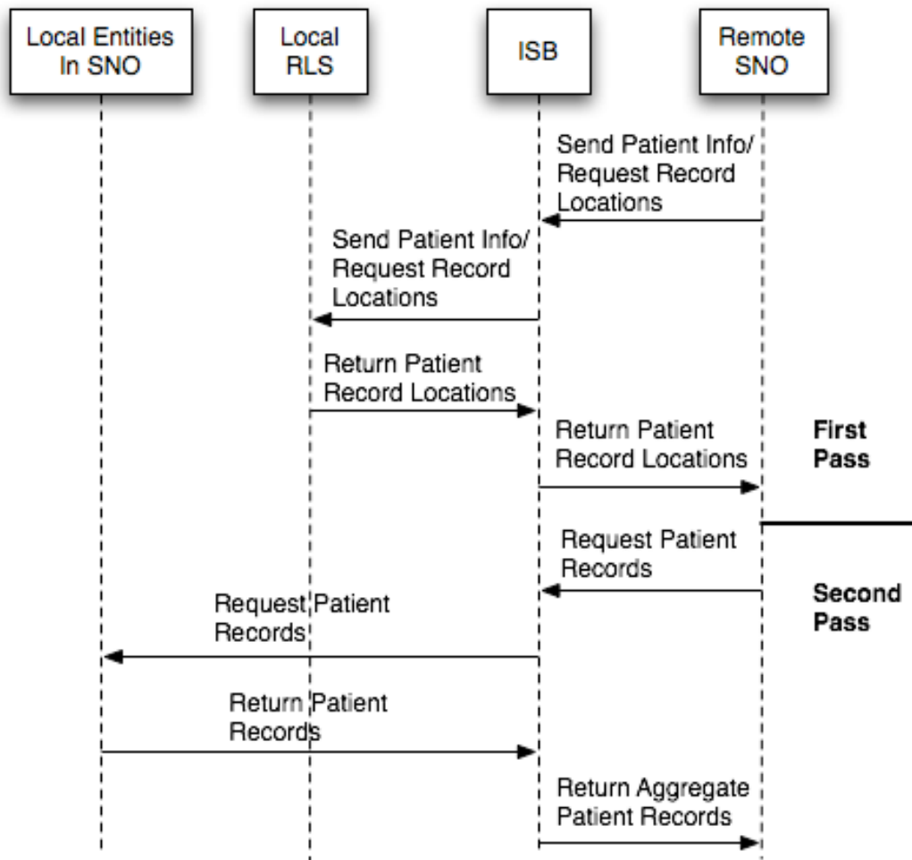
Figure 2 ISB Two Pass Interactions
