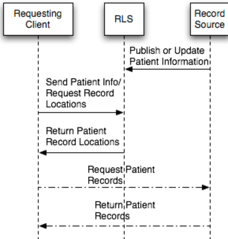
Figure 1 RLS Interactions
