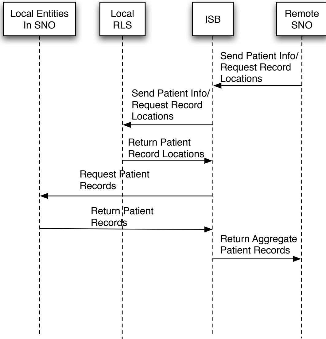
Figure 3 ISB One Pass Interactions
