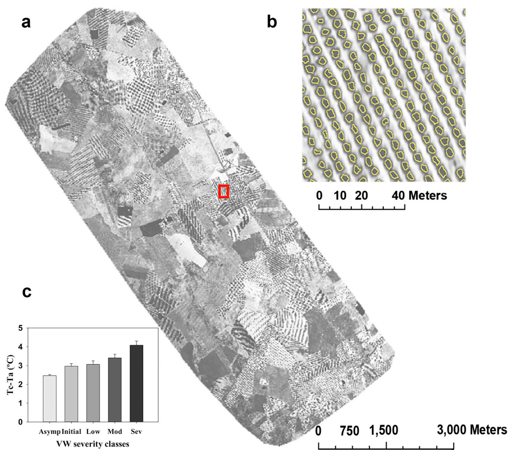
Figure 3. Thermal mosaic (a) obtained with the thermal camera on board the manned platform at 63-cm resolution, enabling pure olive crown identification (b). Pure olive crowns were identified using automatic object-based crown detection. Mean crown normalized temperature ( T_c - T_a ) calculated from thermal imagery is shown for every Verticillium wilt severity class in (c). Mean values of T_c - T_a were supported by the data of the 9 plots, consisting of 510, 98, 64, 46 and 38 olive trees which correspond to asymptomatic, initial, low, moderate and severe severity classes, respectively. Error bars indicate standard errors. Red square (a) is shown in detail in (b).
