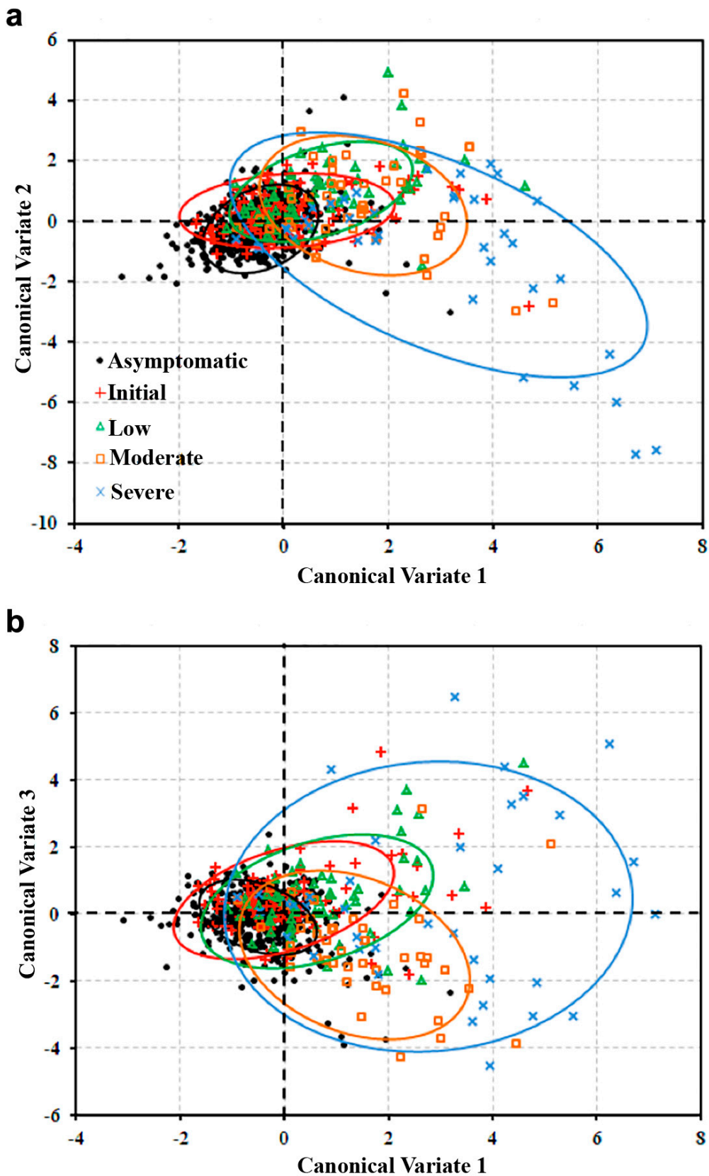
Figure 5. Classification of 756 olive trees assessed in Ecija into five Verticillium wilt severity classes based on (a) the first and second canonical variates and (b) the first and third canonical variates, from the canonical discriminant analysis.
