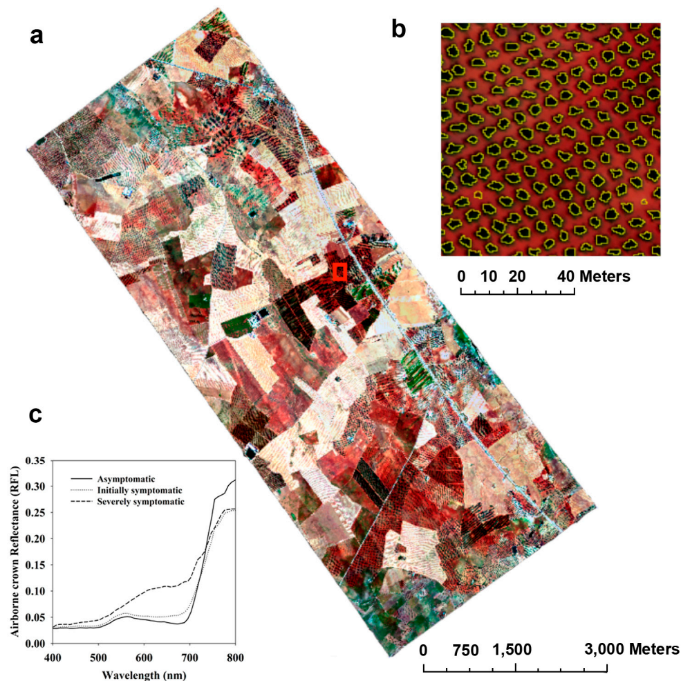
Figure 4. Hyperspectral mosaic (a) obtained with the hyperspectral sensor on board the manned platform at 50-cm resolution. Pure olive crowns were identified using automatic object-based crown detection (b). Sample crown reflectance obtained by the hyperspectral imagery from Verticillium wilt asymptomatic, initially symptomatic and severely symptomatic olive trees is shown in (c). Red square (a) is shown in detail in (b).
