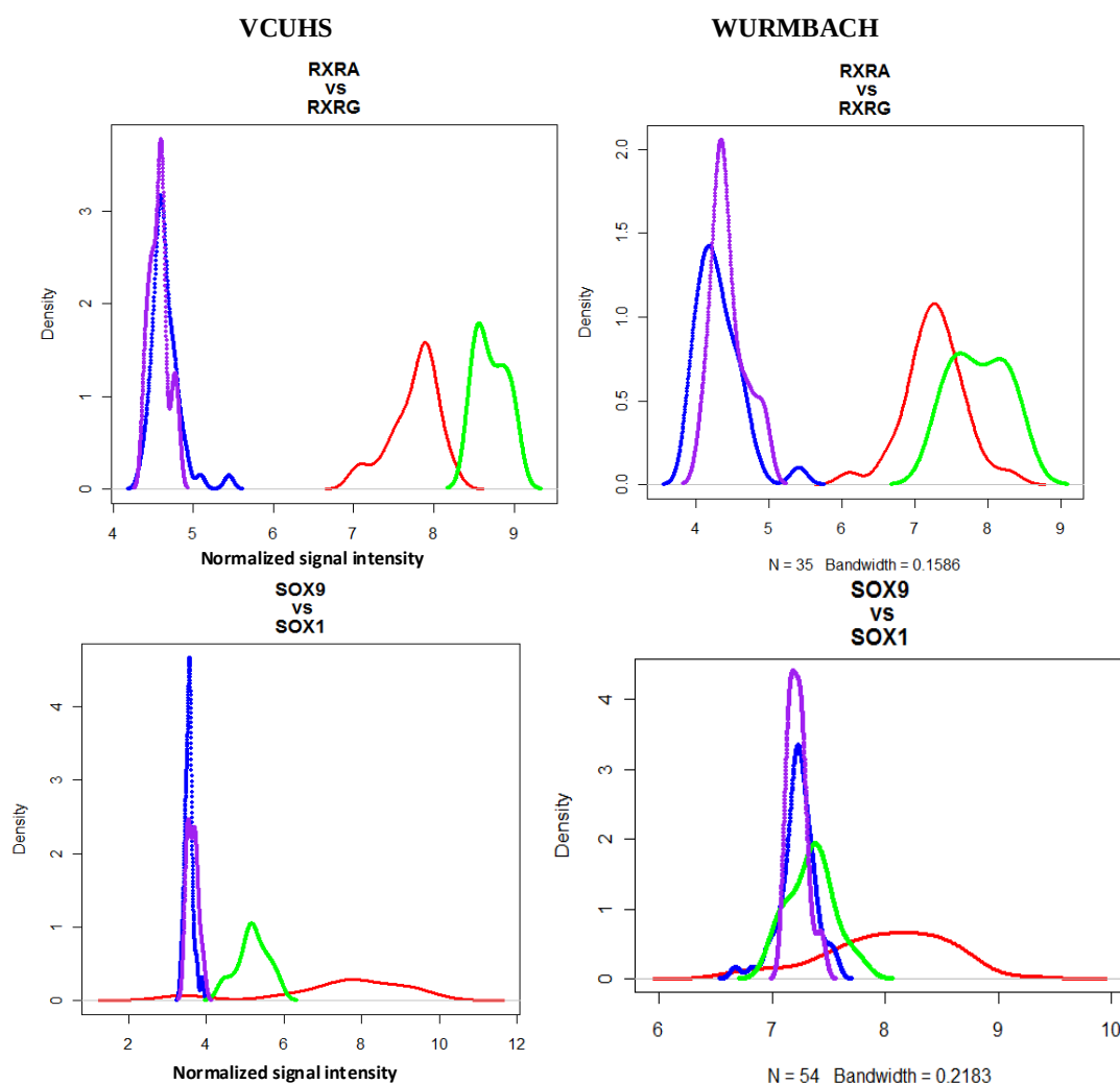
Figure 1. Selected density plots of liver development vs. paralog non-liver development genes. Expression densities are shown for gene pairs in normal and HCC samples from our data and in the Wurmbach dataset. Red = expression of the liver gene in HCC; Green = expression of liver gene in normal controls; Blue = expression of non-liver gene in HCC; Purple = expression of non-liver gene in normal controls. Paralog genes ( RXRG and SOX1 ) were not expressed in HCC or normal samples, while liver development genes RXRA and SOX9 were differentially expressed in HCC. These patterns were also observed in the Wurmbach dataset.
