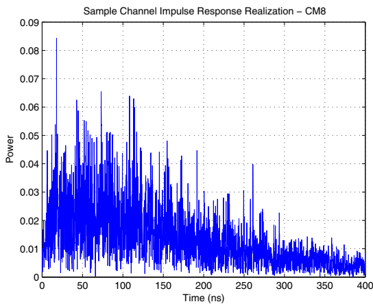
Fig. 2. Impulse response realization in CM8 (industrial NLOS).
