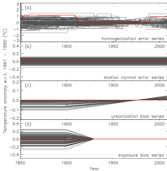
Figure 3 – 100 realizations of each uncertainty component contributing to the CRUTEM4 ensemble realizations, with an example realization of each component highlighted in red. Homogenization and station normal error realizations are drawn for each individual station record. Urbanization bias instances apply globally. Different values of exposure bias are applied uniformly across the extratropics (shown) and the tropics.
