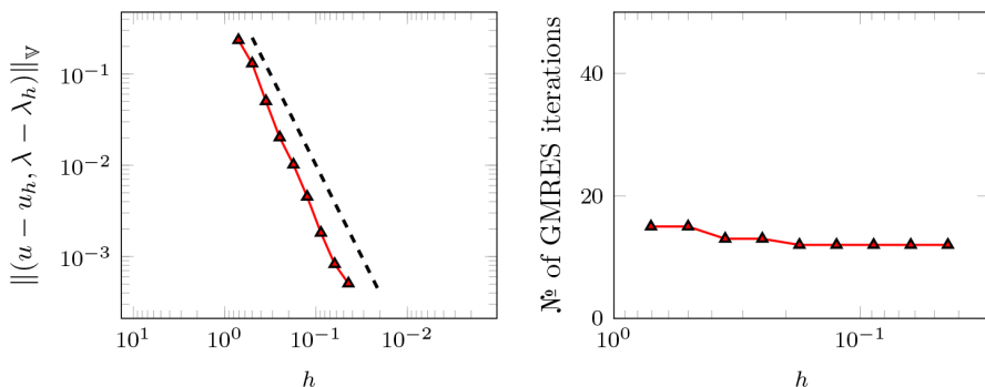
FIG. 5. The error (left) and GMRES iteration counts (right) of the penalty method with \beta_D = 1 - i for the Helmholtz Dirichlet problem with k = 3 on the unit sphere as we reduce h . The dashed line shows order 2 convergence. Here we take (u_h, \lambda_h), (v_h, \mu_h) \in P_h^1(\Gamma) \times P_h^1(\Gamma) and solve to a GMRES tolerance of 10^{-5} .
