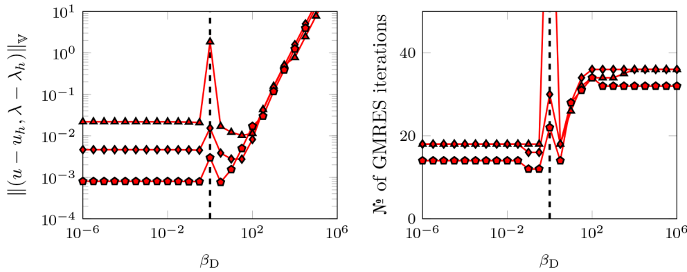
FIG. 2. The error (left) and GMRES iteration counts (right) of the penalty method with varying real \beta_D for the Helmholtz Dirichlet problem with k = 2.759 on the unit sphere with h = 2^{-2} (red triangles), h = 2^{-3} (red diamonds), and h = 2^{-4} (red pentagons). Here we take (u_h, \lambda_h), (v_h, \mu_h) \in P_h^1(\Gamma) \times P_h^1(\Gamma) and solve to a GMRES tolerance of 10^{-5} .
