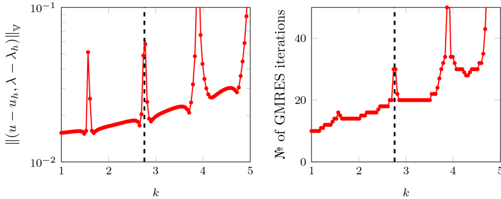
FIG. 1. The error (left) and GMRES iteration counts (right) of the penalty method with \beta_D = 1 for the Helmholtz Dirichlet problem with varying k on the unit sphere with h = 2^{-2} . Here we take (u_h, \lambda_h), (v_h, \mu_h) \in P_h^1(\Gamma) \times P_h^1(\Gamma) and solve to a GMRES tolerance of 10^{-5} .
