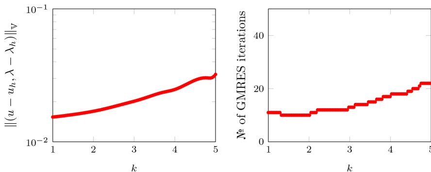
FIG. 4. The error (left) and GMRES iteration counts (right) of the penalty method with \beta_D = 1 - i for the Helmholtz Dirichlet problem with varying k on the unit sphere with h = 2^{-2} . Here we take (u_h, \lambda_h), (v_h, \mu_h) \in P_h^1(\Gamma) \times P_h^1(\Gamma) and solve to a GMRES tolerance of 10^{-5} .
