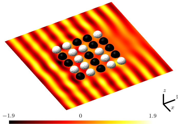
FIG. 6. The incident wave u^{\text{inc}} = e^{ik\mathbf{x}\cdot\mathbf{d}} , where \mathbf{d} = (0, 1, 0) and k = 2 , scattering off 25 spheres. The white spheres are sound-hard and the black spheres are sound-soft.
