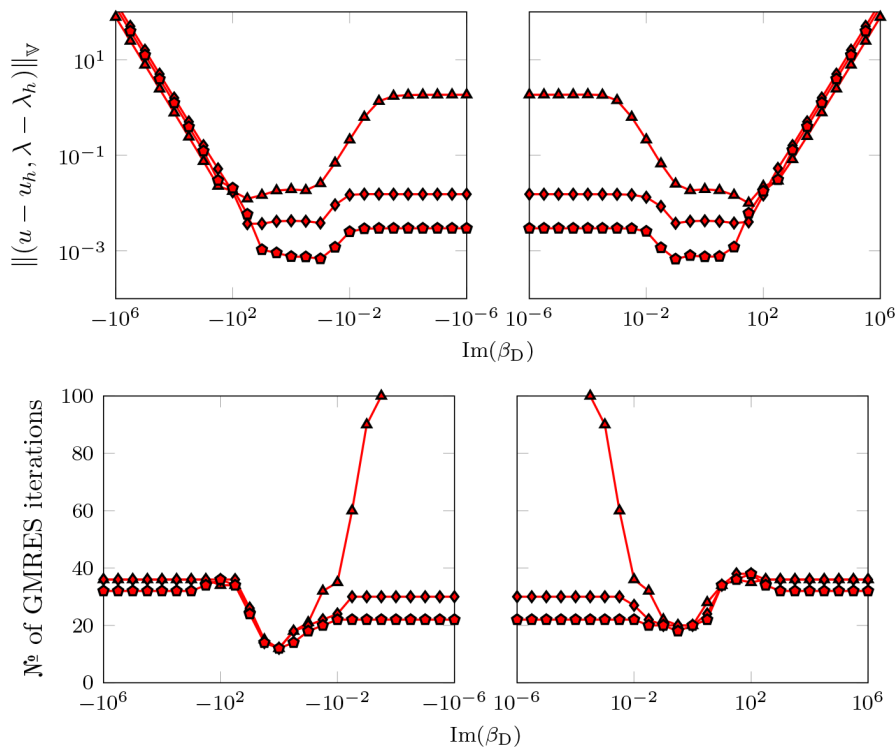
FIG. 3. The error (top) and GMRES iteration counts (bottom) of the penalty method with varying \beta_D with \text{Re}(\beta_D) = 1 for the Helmholtz Dirichlet problem with k = 2.759 on the unit sphere with h = 2^{-2} (red triangles), h = 2^{-3} (red diamonds), and h = 2^{-4} (red pentagons). Here we take (u_h, \lambda_h), (v_h, \mu_h) \in P_h^1(\Gamma) \times P_h^1(\Gamma) and solve to a GMRES tolerance of 10^{-5} .
