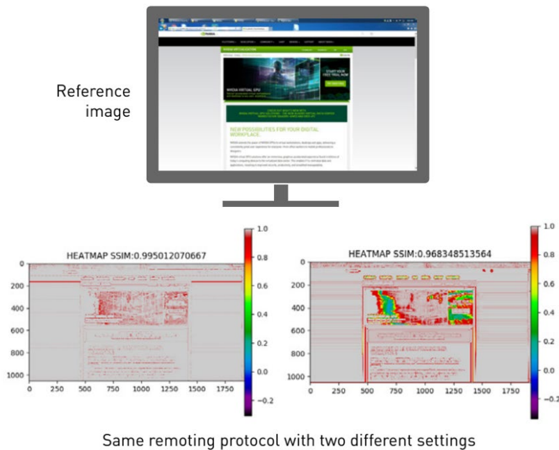
Figure 2-2. SSIM as Measure of Image Density
