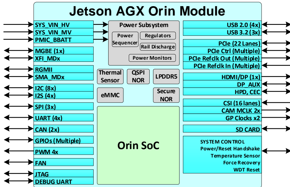
Figure 3: Jetson AGX Orin Series System-On-Module
