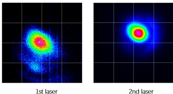
Figure 6: Beam profile.
