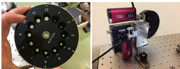
Figure 5: Aperture setting.
