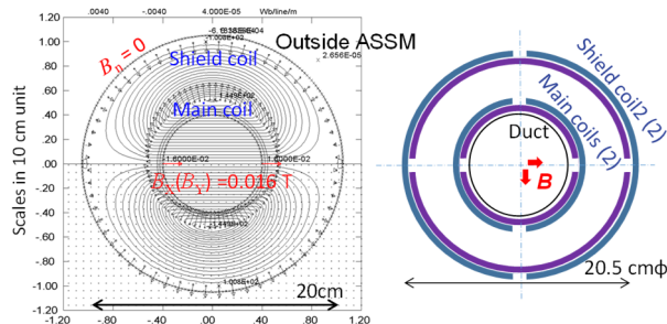
Figure 4: Left shows result of 2D design calculations for outside-ASSM. Lines: Flux contour lines at every 40 \mu Wb/m. Arrows: current magnitudes. Right schematic coil assemble plan of two dimensional ASSM.
