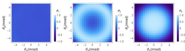
Figure 4: Spatial distribution of the normalized Stokes parameters at \psi_0 = \pi/2 . The left, the middle and the right figure show P_1 , P_2 , and P_3 , respectively.
