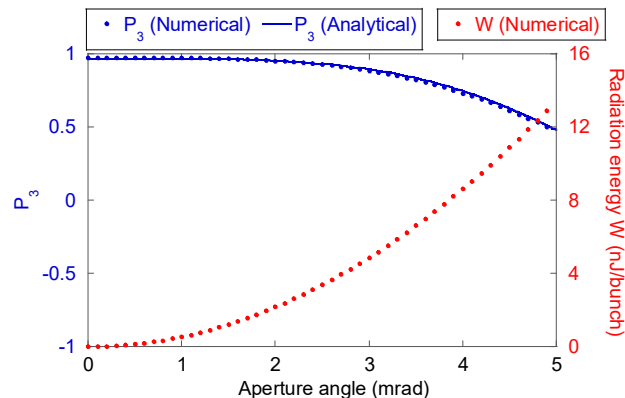
Figure 5: P_3 (blue) and normalized radiation energy (red) within a circular aperture. The dots and solid line denote numerical calculation and analytical calculation, respectively.
