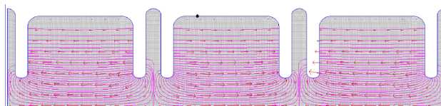
Figure 2: APS cavity.
