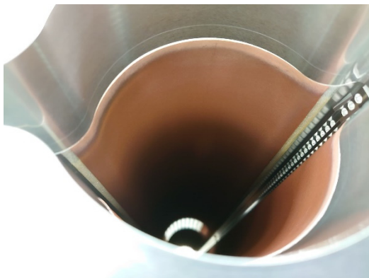
Figure 10: The high temperature caused by welding discolored the surrounding coating.
