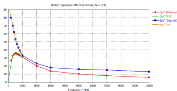
Figure 5: Permittivity of a SiC, \epsilon' : blue, and \epsilon'' : red.
