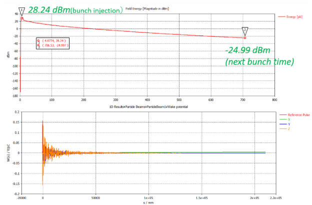
Figure 7: Calculated field energy (A) and wake potential (B) during one-bunch time separation of 700 ns.
