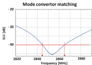
Figure 4: Matching characteristics of the mode convertor from the rectangular wave guide TE10 mode to the circular wave guide TE11 mode.
