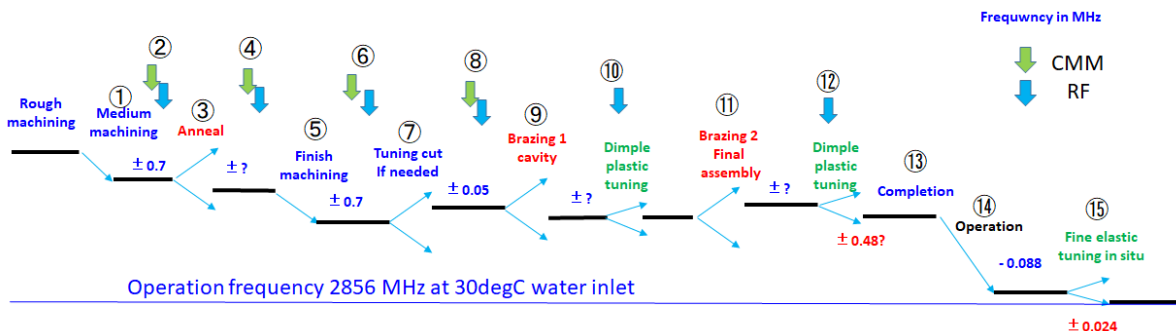
Figure 3: Control idea of the cavity resonant frequency through all the fabrication stages and until full-power operation.
