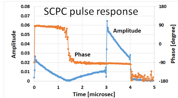
Figure 15: Typical pulse response of the SCPC system.
