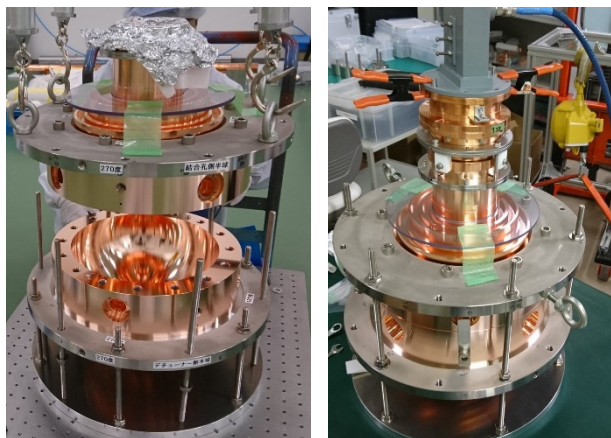
Figure 5: Left: Two hemispheres are being set to make a spherical cavity, right: mode convertor is set on top of the circular wave guide, ready to measure cavity resonance from circular wave guide.
