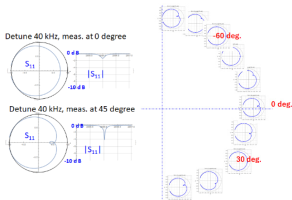
Figure 6: S11 reflection measurement of the cavity mode by the setup in Fig. 5. Left: examples of two lightly degenerate modes seen from a mode convertor set at 0 and 45 degrees w.r.t. one of the modes.
