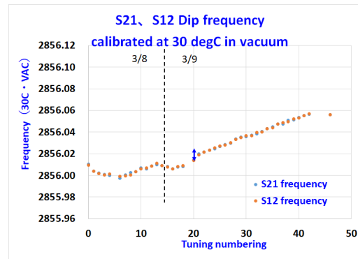
Figure 14: Variation of cavity resonant frequency through whole tuning history.
