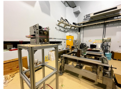
Figure 10: Setup of magnetic field measurement.
