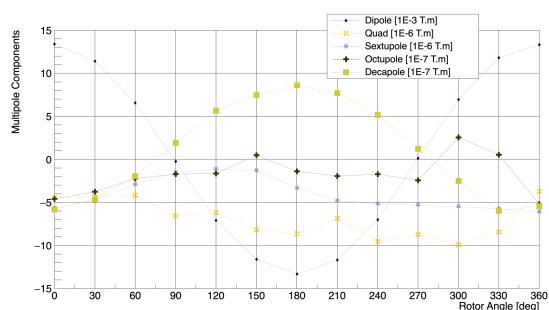
Figure 15: Integrated multipole components from measured data as functions of rotation angle of the rotor.
