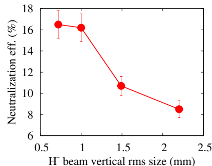
Figure 11: Neutralization dependence on the vertical size of the \text{H}^- beam. A maximum efficiency of 16.5% was obtained by minimizing the beam size to 0.72 mm.
