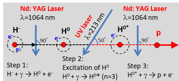
Figure 1: Schematic view of the concept of H^- stripping to proton by using only lasers. Noted laser parameters are for 400 MeV H^- beam stripping.
