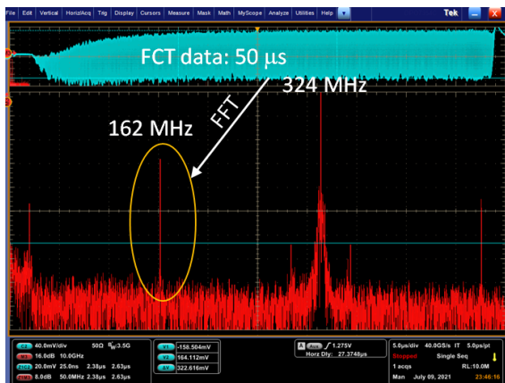
Figure 6: Online confirmation of laser and H^- beam interaction by FFT analysis of the FCT time domain data for a signal at 162 MHz as the neutralization occurred for every alternate H^- beam pulses.
