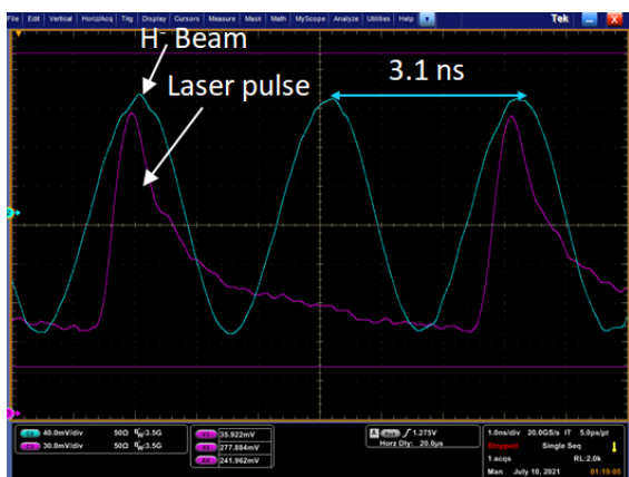
Figure 5: Laser pulse (purple) synchronized to every alternate H^- micro pulses (sky blue).
