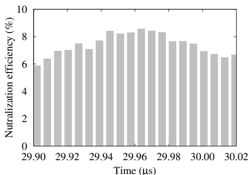
Figure 9: Neutralization efficiency of several pulses at around at around 30 \mu\text{s} of the \text{H}^- pulse, the maximum efficiency was 8.5% and in average it was (7.4 \pm 0.8)\% .
