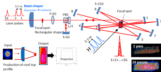
Figure 3: Schematic view of the newly developed multi-reflection laser cavity system to reduce the seed laser power. A beam shaper is used to transform a Gaussian to uniform laser pulse before transferring to the cavity.
