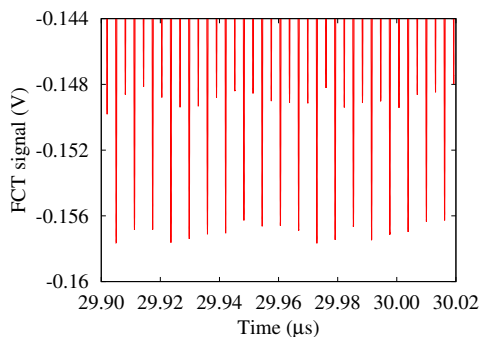
Figure 8: Expanded view of the FCT time domain signal of H^- at the central region. The height of every alternate pulses reduced due to the neutralization with laser interaction.
