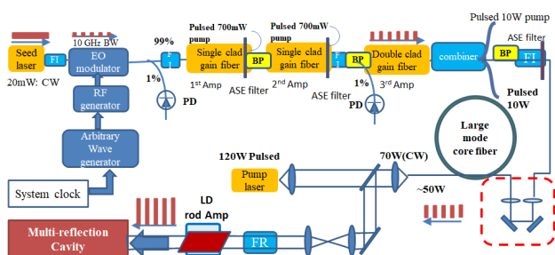
Figure 2: Schematic view of under development prototype YAG laser system for the POP demonstration.
