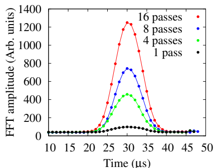
Figure 10: FFT amplitudes of 162 MHz of the FCT data with respect to the number of laser passes in the cavity. The efficiency increases by increasing the laser pulse energy at the IP with number of passes.
