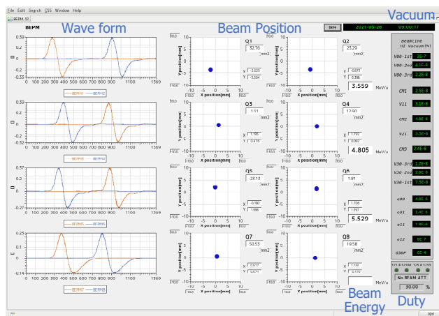
Figure 4: An example of the displayed measurement panel programmed with CSS on EPICS when the ^{51}\text{V}^{13+} beam was accelerated. From left to right, the beam signal waveforms, beam positions, beam energies, vacuums, and duty of chopped beam are shown.
