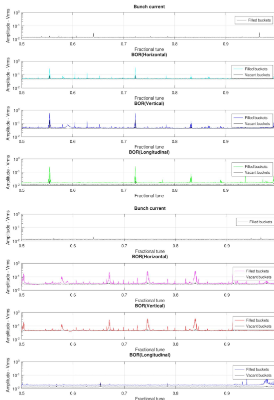
Figure 4: Average spectra of filled buckets compared to that of empty buckets of HER (upper) and LER (lower) for a manual abort.
