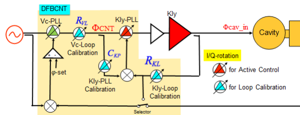
Figure 2: Block diagram of phase control in digital LLRF control system.
