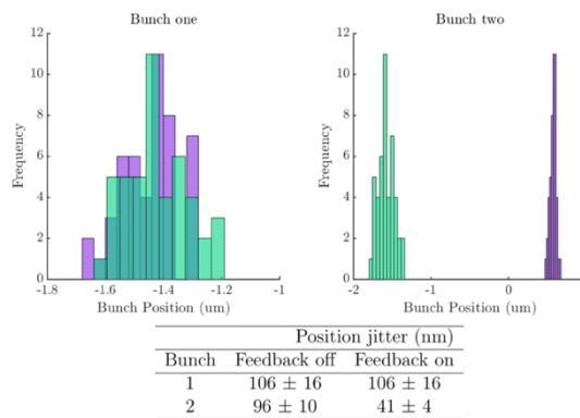
Figure 10: Beam position at IP BPM w/wo FONT.
