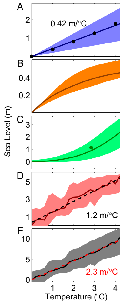
Fig. 2. Sea-level commitment per degree of warming as in Fig. 1 except for sea-level contributions after 2,000 y. Results were obtained from physical model simulations of (A) ocean warming, (B) mountain glaciers and ice caps, and (C) the Greenland and (D) the Antarctic Ice Sheets. (E) The corresponding total sea-level commitment. Temperatures are relative to preindustrial. Dashed lines and large black dots provide linear approximations: (A) sea-level rise for a homogeneous increase in temperature; (D and E) constant slopes of 1.2 and 2.3 m/°C. Shading represents the uncertainty range as discussed in the text. The large green dot in C corresponds to the sea-level contribution of Greenland (following ref. 3) after 1,000 y of integration with 560 ppm atmospheric CO 2 concentration and a standard polar amplification of 1.5, which translates Greenland temperatures to the global mean temperature.
